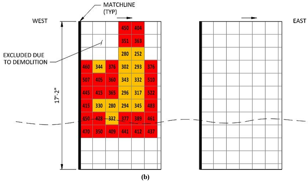
(b) Figure 14. Half-Cell Measurements Using a 16-x-16-Inch Grid Pattern Show a Probability of Corrosion on the (a) Pier 1 and (b) Pier 4 Columns of the Route 522 Bridge. Numbers in each square are the magnitude of the half-cell measurement but are reported as positive values instead of the measured negative value. The dashed line indicates approximate ground level location (VDOT Contracted I-64 Bridge Substructure Studies Project, Route 522, 2021).
