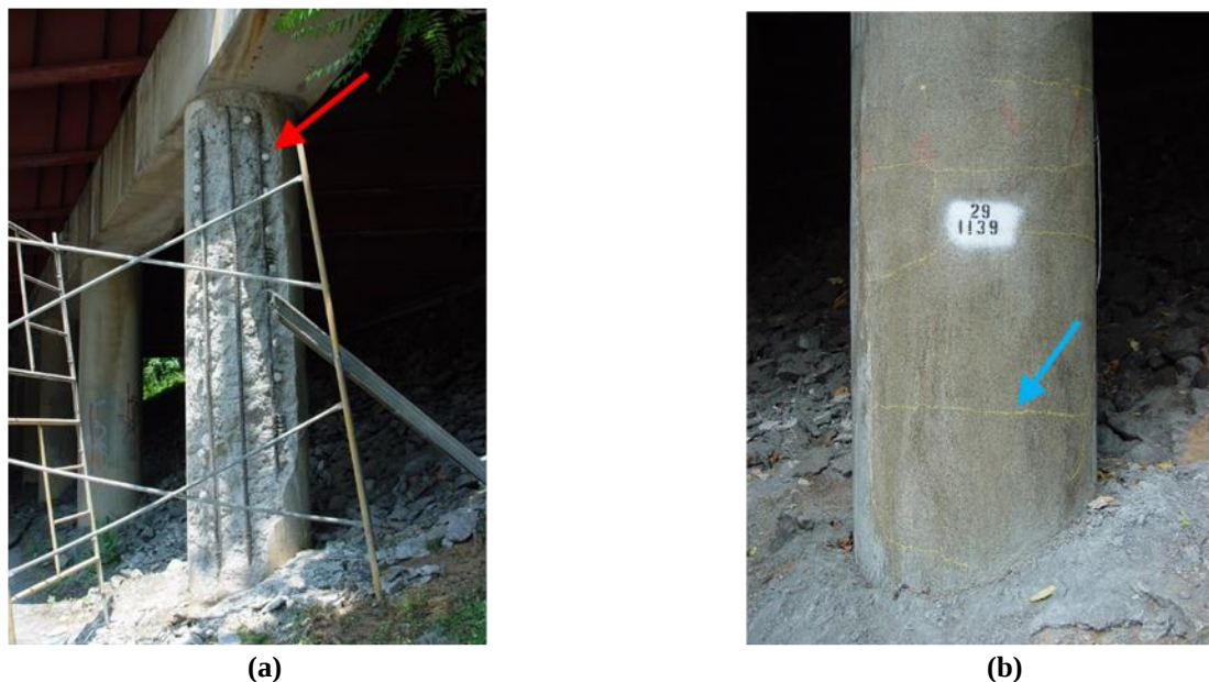
Figure 1. Placement of Anodes in Shotcrete Repair Area: (a) Column with DPG anodes (red arrow) tied to steel prior to shotcrete repair and (b) after shotcrete hardens and exhibits shrinkage cracks (blue arrow) that were emphasized on the column using yellow crayon. The cracks widths marked in yellow are less than 0.01 inch (Brown and Sharp, 2005).
