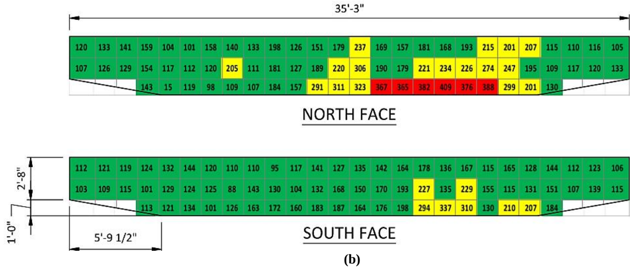
Figure 17. Half-Cell Measurements Using a 16-x-16-Inch Grid Pattern Show a Probability of Corrosion on the (a) Pier 1 and (b) Pier 4 Caps of the Route 621 Bridge. Numbers in each square are the magnitude of the half-cell measurement but are reported as positive values instead of the measured negative value (VDOT Contracted I-64 Bridge Substructure Studies Project, Route 621, 2021).
